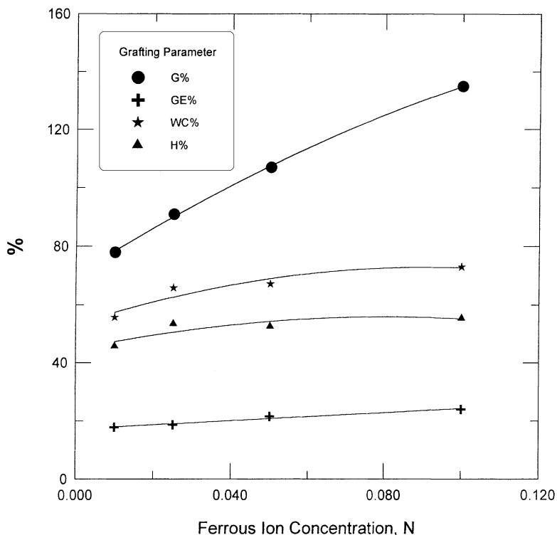
FIGURE 5 Effect of cation [\text{Fe}^{+2}] on grafting of acrylic acid onto cellophane films. [\text{H}_2\text{O}_2] , 0.025%; [\text{AA}] , 25%; Time, 4 hrs; Temp. 60^\circ\text{C} .
